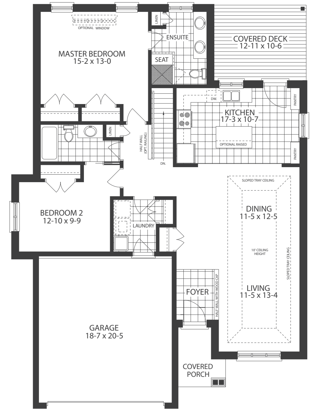
MAIN FLOOR ELEVATION A
