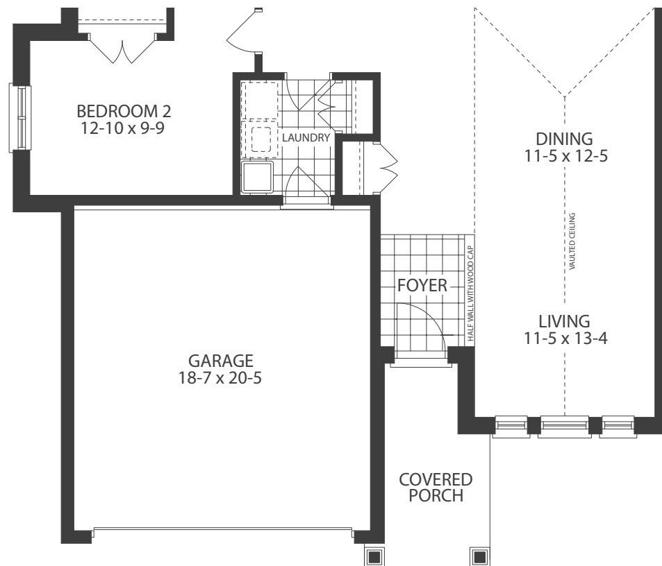
MAIN FLOOR ELEVATION B
